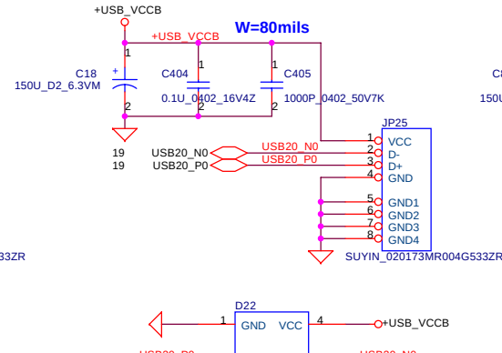
USB CONN. 3 & 5 (Place on the right side)
