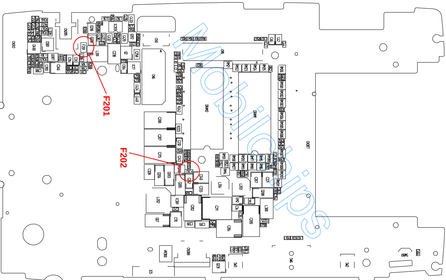
BOTTOM VIEW
