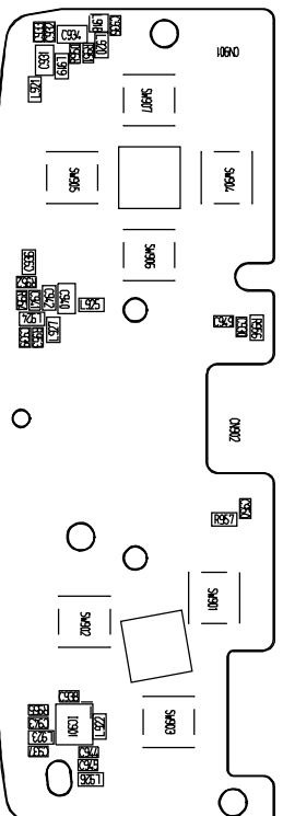
TOP VIEW
