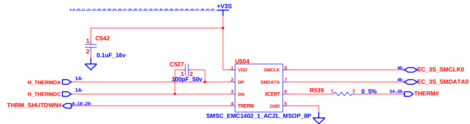
Thermal Sensor For CPU
