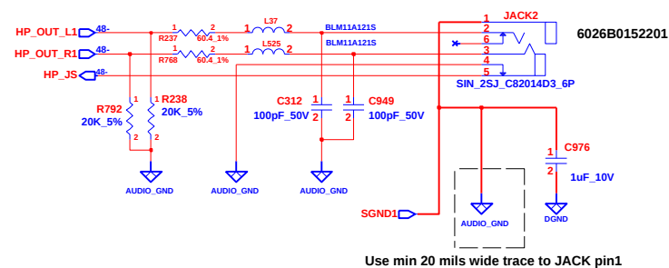
Earphone Jack
