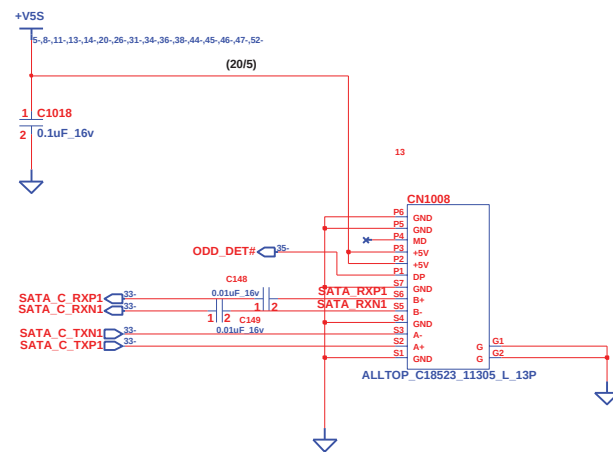
SATA ODD
