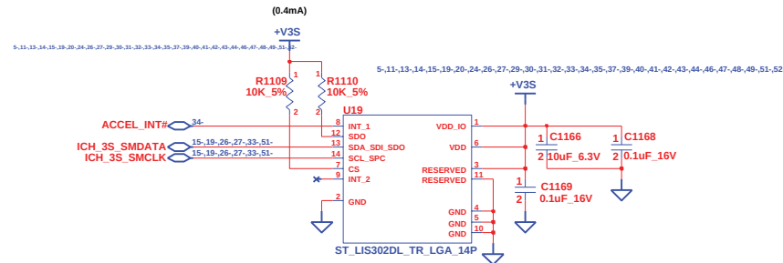
Accelerometer
