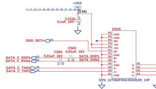
SATA ODD
