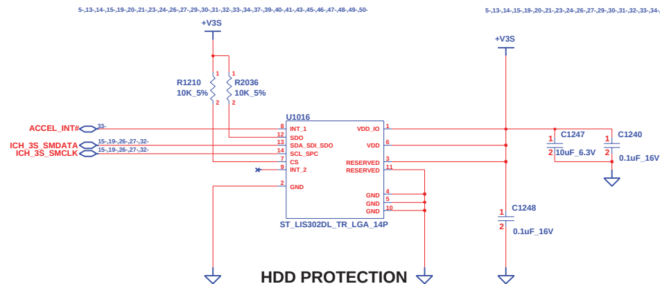
HDD PROTECTION
