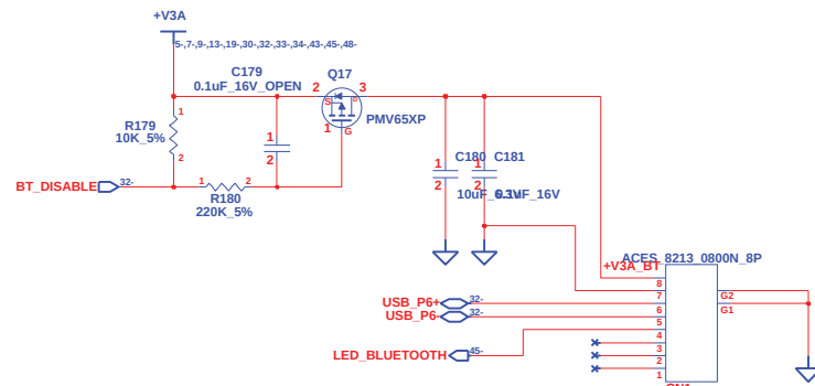
BLUETOOTH CNTR
